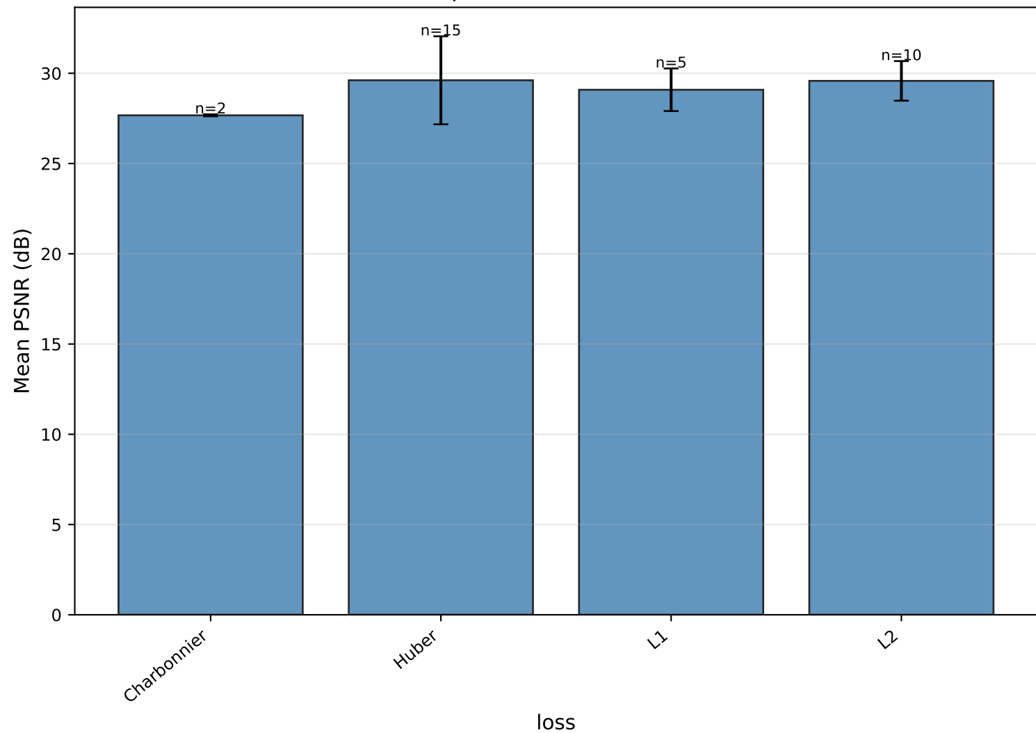
Mean PSNR per value of loss — SRFormer
